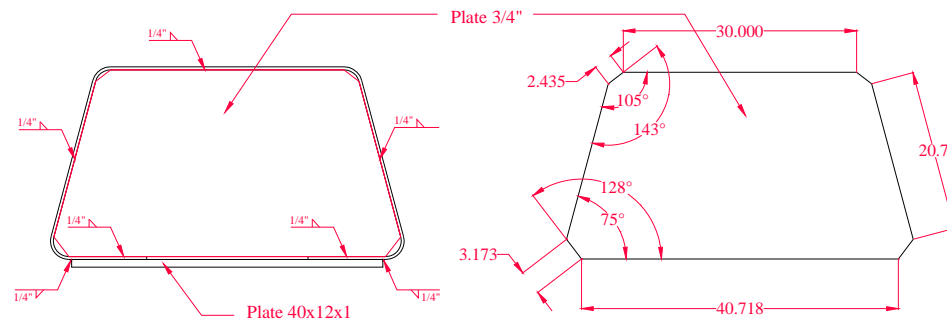
Figure 2-3 Girder bearing plate and stiffener dimensions
