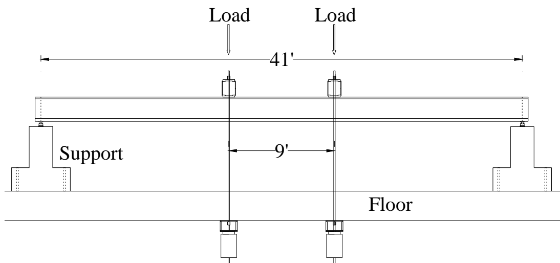
Figure 2-6 Test setup
