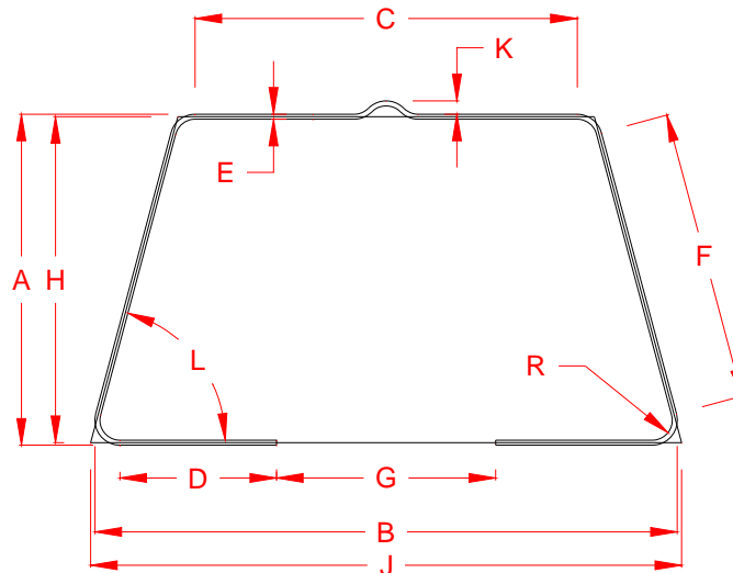
Figure 1-1 Folded plate girder cross section
