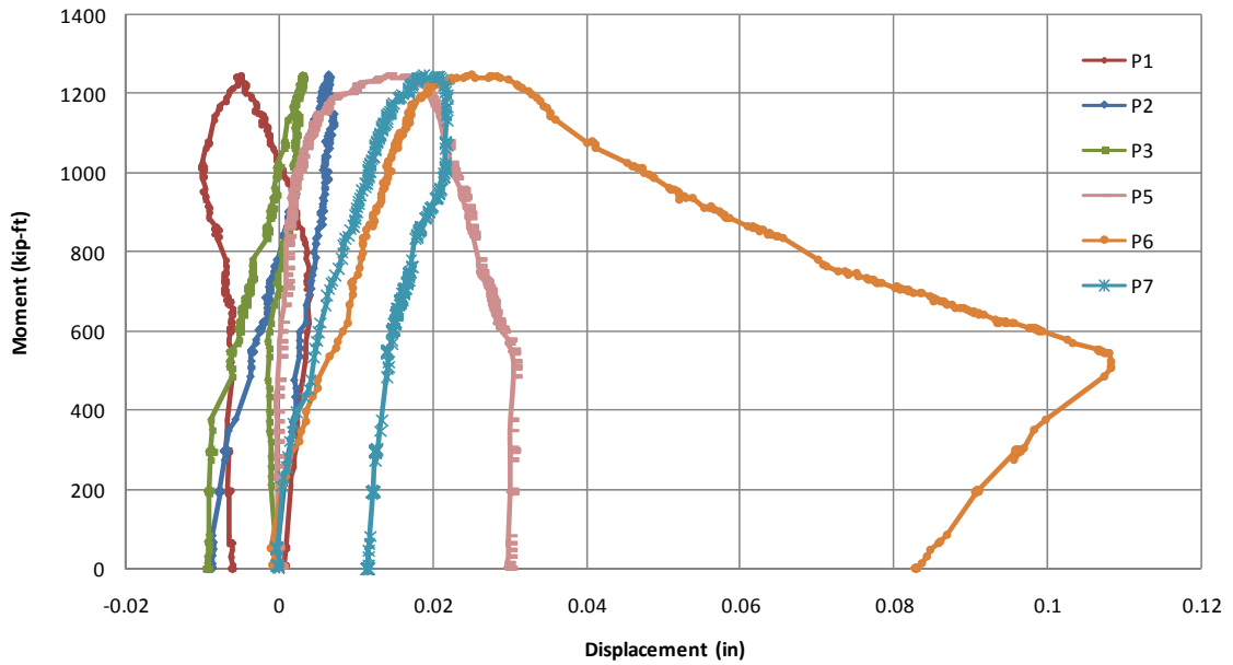
Figure 3-51 Flange separation moment-displacement graph
