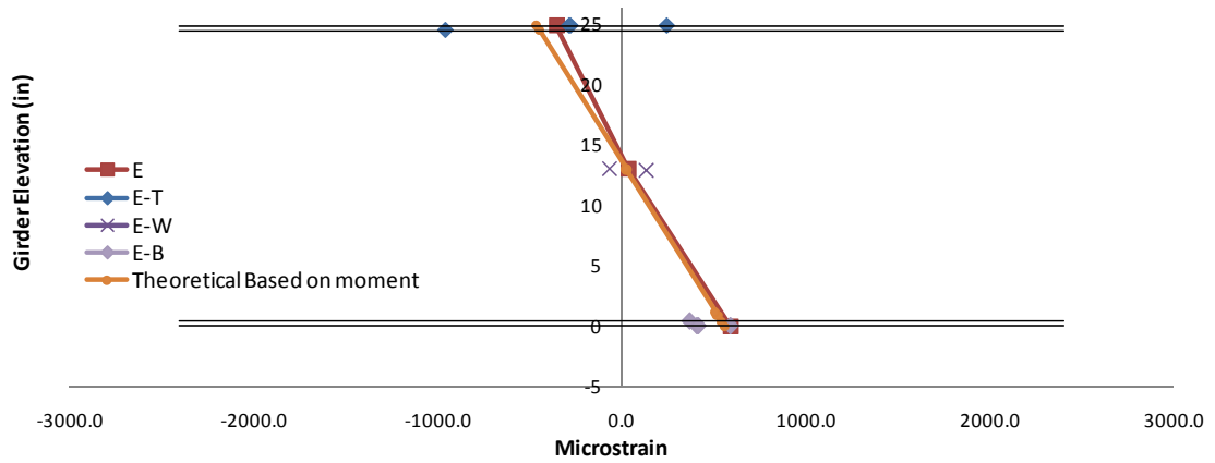
Figure 3-28 Section E strain distribution at 2 times construction moment
