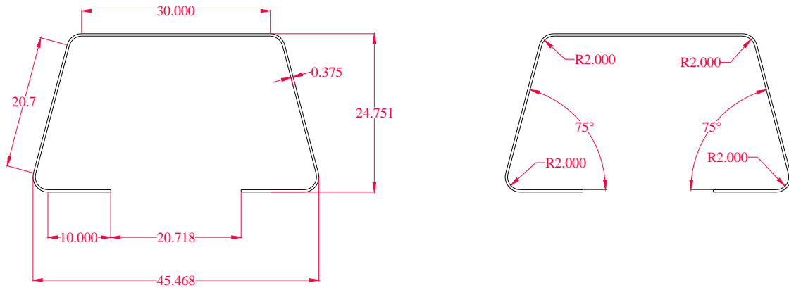
Figure 2-2 Folded plate geometry
